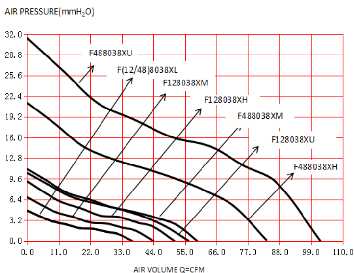
AIR FLOW-AIR PRESSURE(PERFORMANCE CURVES)
